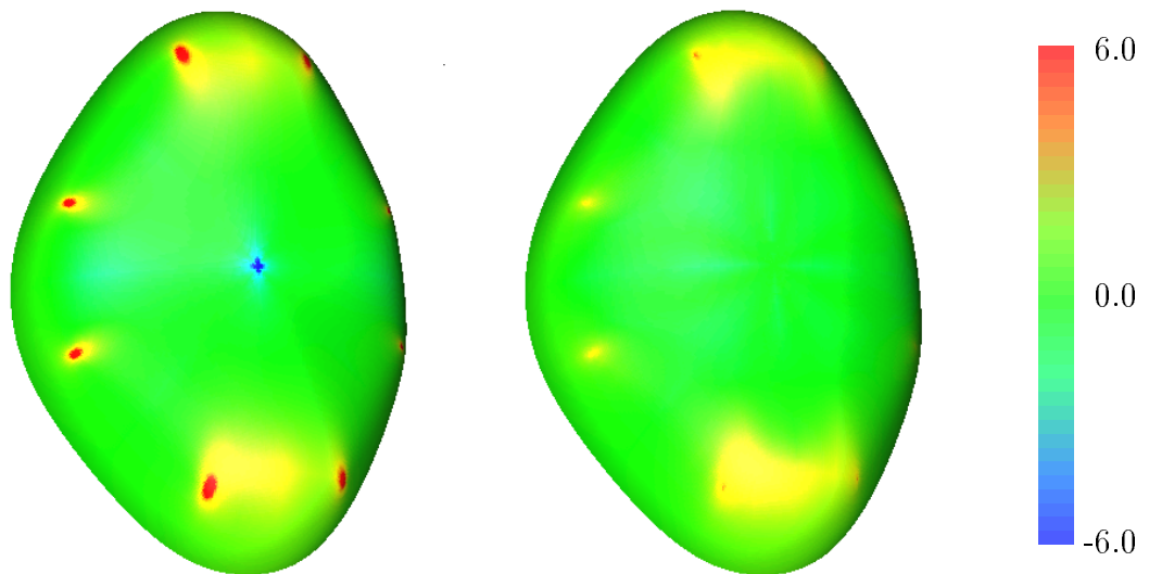
Figure 6: The surfaces produced by the Catmull/Clark algorithm (left) and its modification (right).
